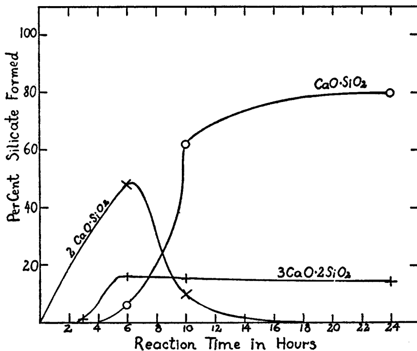
FIG. 18. Sequence of compound formation in system CaO + SiO 2 (Jander and Hoffmann (94)).
