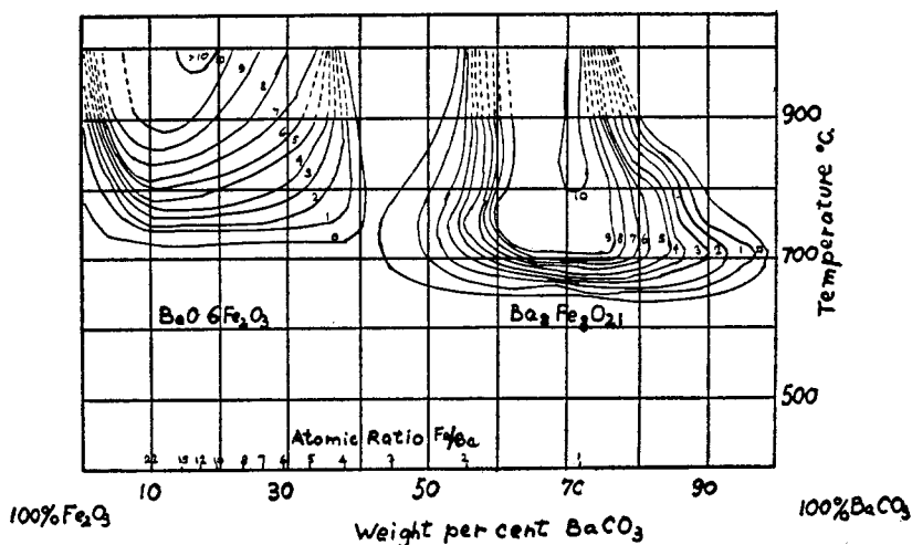
FIG. 19. Formation of \text{BaO} \cdot 6\text{Fe}_2\text{O}_3 and \text{Ba}_3\text{Fe}_3\text{O}_{21} in system \text{BaCO}_3 + \text{Fe}_2\text{O}_3 (Erbak, Fankuchen, and Ward (26)).
