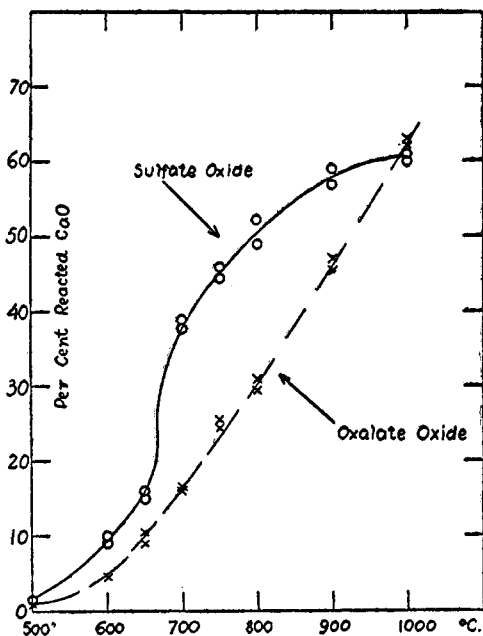
FIG. 14. Significance of parent substance on reactivity of ferric oxide (Hedvall and Sandberg (66)).
