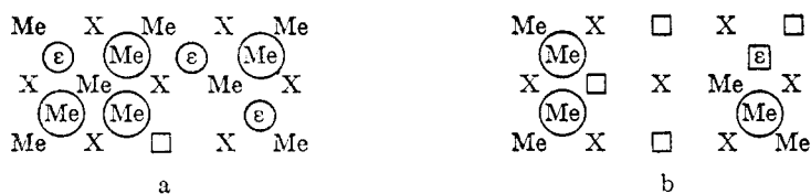
FIG. 10. Illustration of Wagner's method to determine types of disorder
